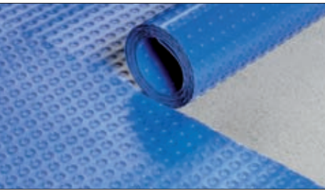
Roll out membrane, studs facing down. Roll out next length and place it edge-to-edge against the adjoining length of membrane.
