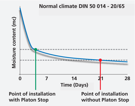
The graph illustrates the drying period for concrete slab (Estrich) and clearly indicates that Platon Stop Original as underlay allows for a much earlier installation of flooring.
