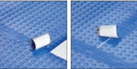
Join connecting edges and details with 75 mm wide Platon Stop Tape.
